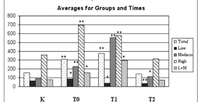
Fig. 2. Averages of the groups low, medium, high and low + medium adherences using the t Student test respect to K, in the different times of virus absorption.
