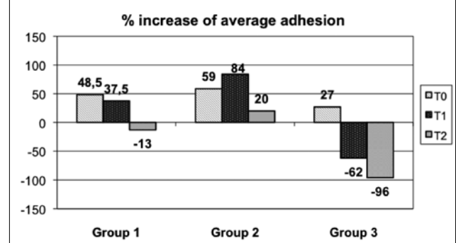
Fig. 1. Percentage increase of average adhesion of the three different groups in T0, T1 and T2.
